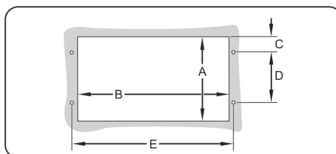
RMB2 Series Cutout Dimensions
