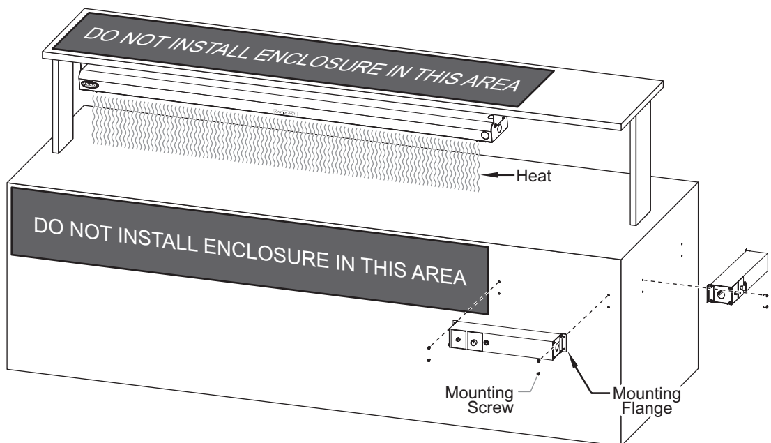
Remote Mounted Enclosure Installation Locations
