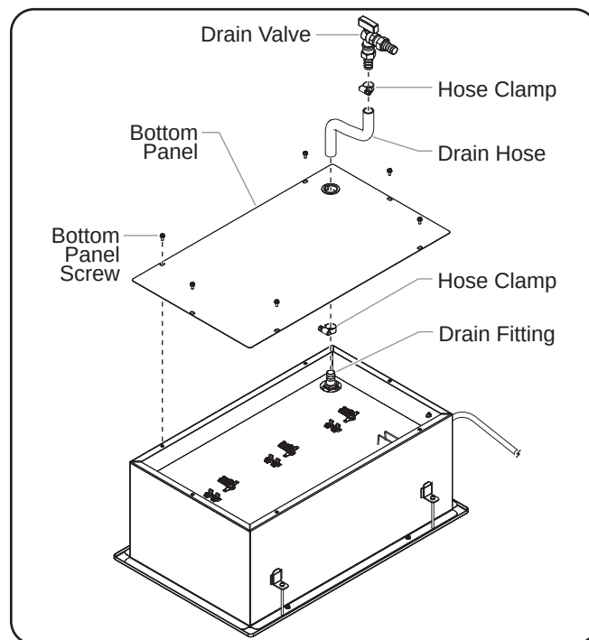
Installing the Drain Assembly (Built-in rectangular models only)
