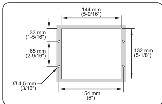
Control Box Cutout Dimensions
