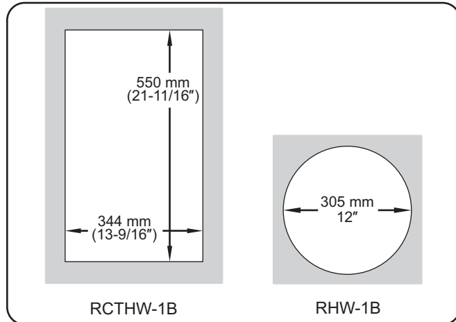
Countertop Cutout Dimensions
