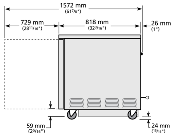
RIGHT VIEW
