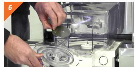
6 Remove the fixing plate and the deposit base.
