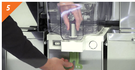
5 Take off the deposit cover and remove the piston and the lever.
